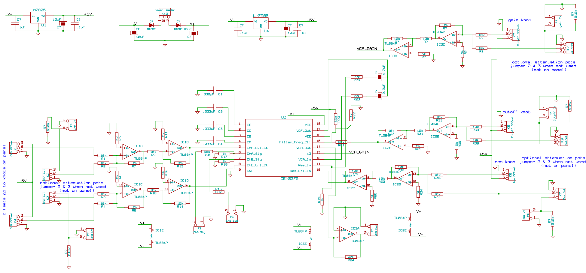
Voice of Saturn CEM3372 Filter r1
